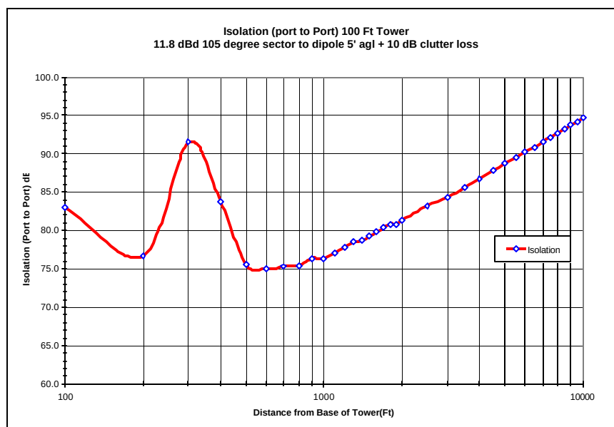
Figure 41 Port-to-Port Isolation
