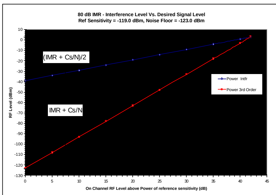
Figure 10 IMR Performance
