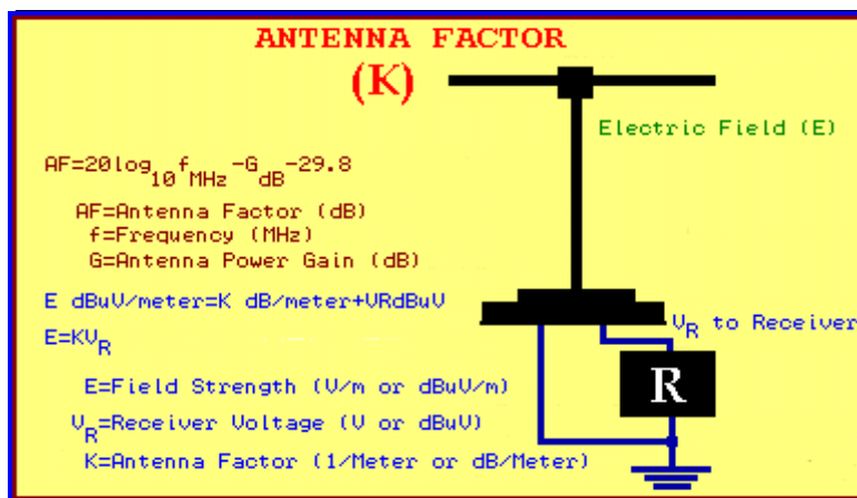
FIGURE 2. ANTENNA FACTOR
