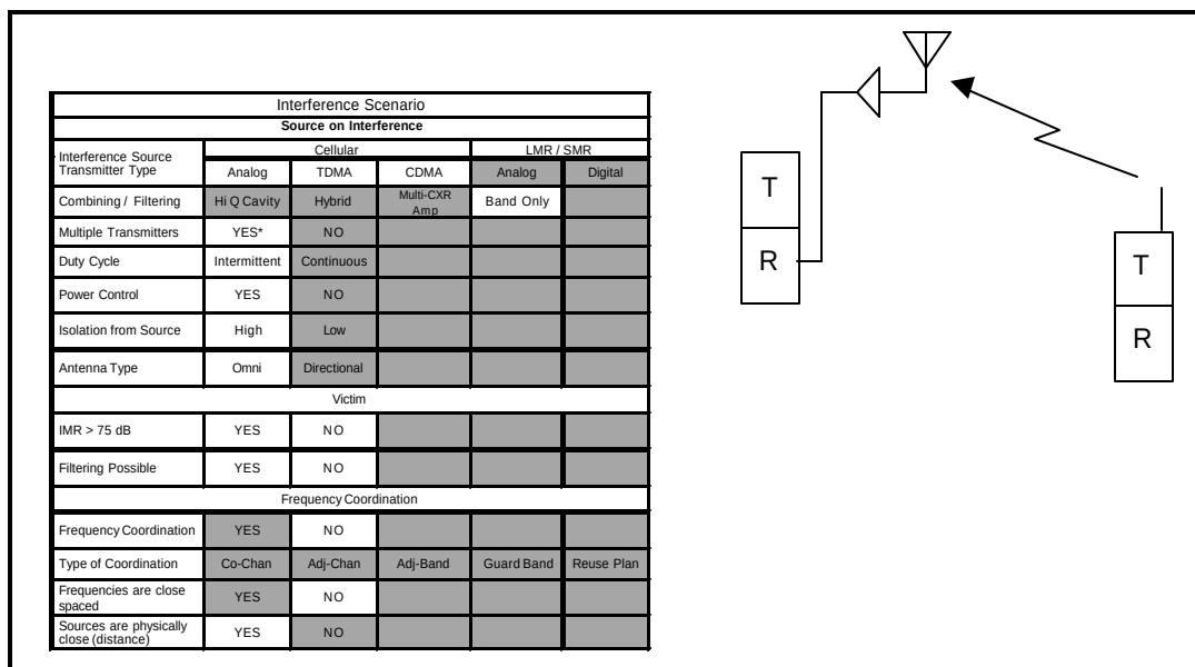
Figure 32 Case 6B, Cellular Subscriber to LMR Base
