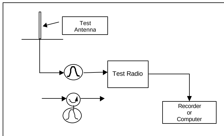
Figure 18 Sideband Noise Determination
