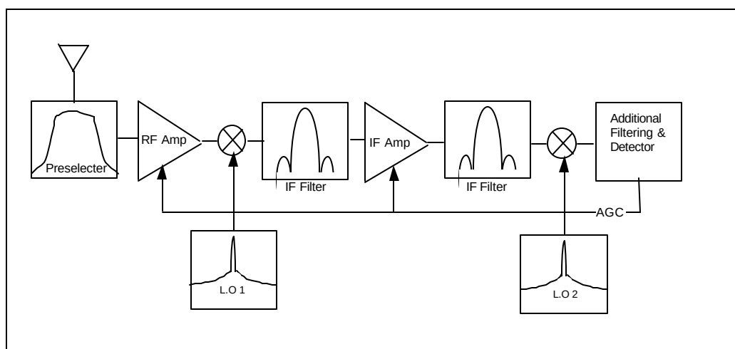
Figure 6 Typical Receiver
