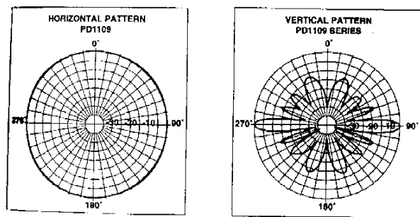
Figure 34 PD 1109 Antenna Pattern.
